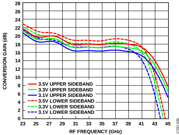
Figure 34. Conversion Gain vs. RF Frequency at Maximum Gain for Various Supply Voltages, f_{IF} = 3.5\text{ GHz} (Upper Sideband and Lower Sideband)
