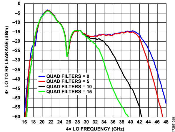
Figure 86. 4× LO to RF Leakage vs. 4× LO Frequency for Four Different QUAD_FILTERS Settings
