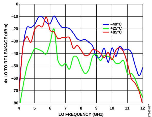
Figure 74. 4x LO to RF Leakage vs. LO Frequency at Various Temperatures (Calibrated). Note: Calibrated at Each Frequency Using MXER\_OFF\_ADJ\_I\_N , MXER\_OFF\_ADJ\_I\_P , MXER\_OFF\_ADJ\_Q\_N , and MXER\_OFF\_ADJ\_Q\_P Bits at T_A = 25^\circ C
