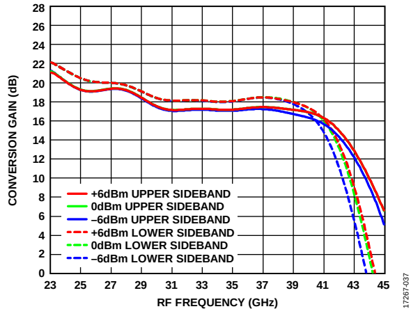
Figure 35. Conversion Gain vs. RF Frequency at Maximum Gain for Various LO Inputs, f_{IF} = 3.5\text{ GHz} (Upper Sideband and Lower Sideband)
