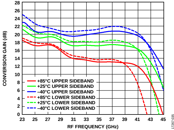
Figure 33. Conversion Gain vs. RF Frequency at Maximum Gain for Various Temperatures, f_{IF} = 3.5\text{ GHz} (Upper Sideband and Lower Sideband)
