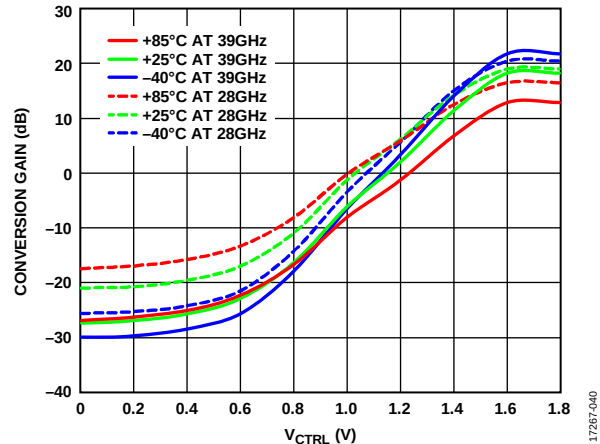
Figure 38. Conversion Gain vs. V_{CTRL} at Various Temperatures at f_{RF} = 28\text{ GHz} and 39\text{ GHz} , f_{IF} = 3.5\text{ GHz} (Lower Sideband)
