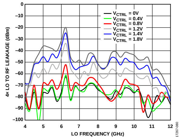
Figure 77. 4x LO to RF Leakage vs. LO Frequency at Various V_{CTRL} (Calibrated) Note: Calibrated at Each Frequency Using MXER\_OFF\_ADJ\_I\_N , MXER\_OFF\_ADJ\_I\_P , MXER\_OFF\_ADJ\_Q\_N , and MXER\_OFF\_ADJ\_Q\_P Bits at V_{CTRL} = 1800\text{ mV}
