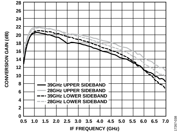
Figure 36. Conversion Gain vs. IF Frequency at f_{RF} = 28\text{ GHz} and 39\text{ GHz} at Maximum Gain (Upper Sideband and Lower Sideband)
