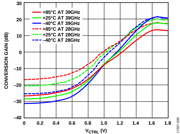
Figure 37. Conversion Gain vs. V_{CTRL} at Various Temperatures at f_{RF} = 28\text{ GHz} and 39\text{ GHz} , f_{IF} = 3.5\text{ GHz} (Upper Sideband)
