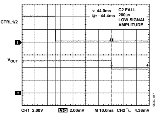
Figure 16. TPC Delay
