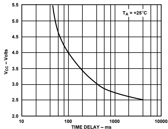
Figure 13. \overline{RESET} Timeout Delay vs. V_{CC}
