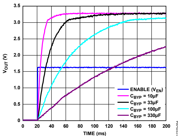
Figure 55. Typical Start-Up Behavior with C_{BYP} = 10 \mu F to 330 \mu F
