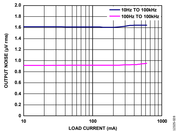
Figure 28. RMS Output Noise vs. Load Current ( I_{LOAD} )
