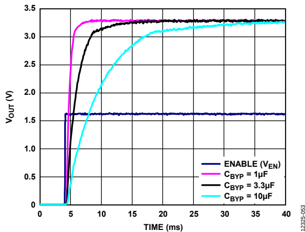
Figure 54. Typical Start-Up Behavior with C_{BYP} = 1 \mu F to 10 \mu F
