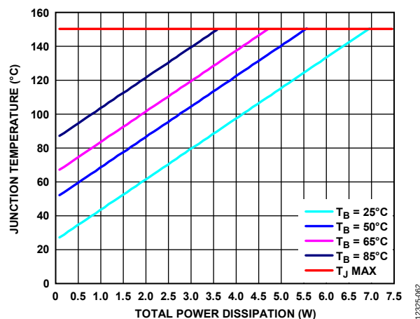
Figure 63. Junction Temperature vs. Total Power Dissipation for the 8-Lead SOIC
