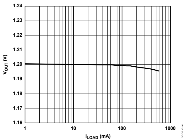
Figure 16. Output Voltage ( V_{OUT} ) vs. Load Current ( I_{LOAD} ), V_{OUT} = 1.2\text{ V}
