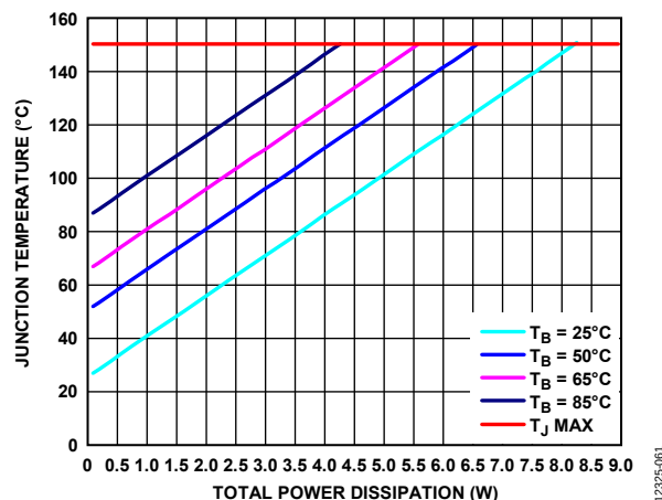
Figure 62. Junction Temperature vs. Total Power Dissipation for the 8-Lead LFCSP
