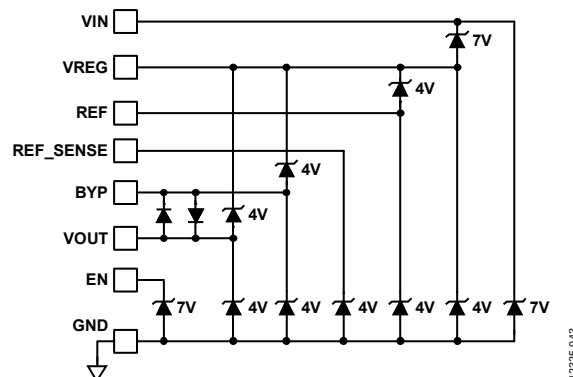
Figure 44. Simplified ESD Protection Block Diagram
