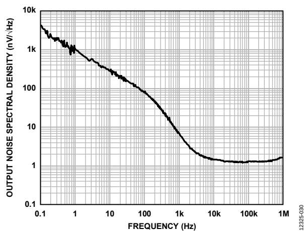
Figure 31. Output Noise Spectral Density, 0.1 Hz to 1 MHz, I_{\text{LOAD}} = 10 \text{ mA}
