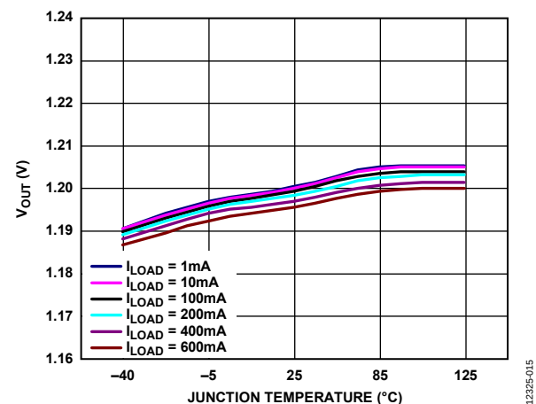
Figure 15. Output Voltage ( V_{OUT} ) vs. Junction Temperature ( T_J ) at Various Loads, V_{OUT} = 1.2\text{ V}
