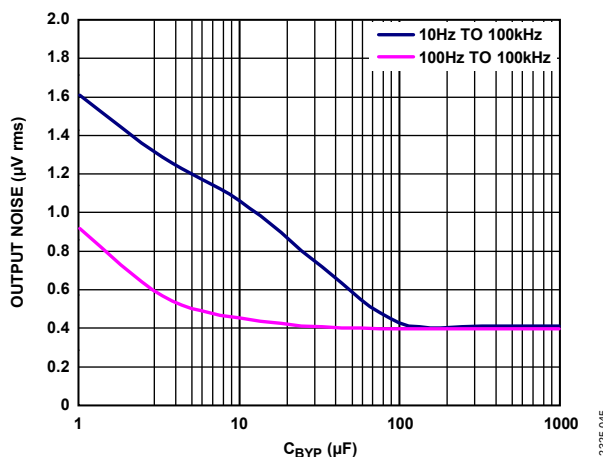
Figure 46. RMS Noise vs. C_{BYP}
