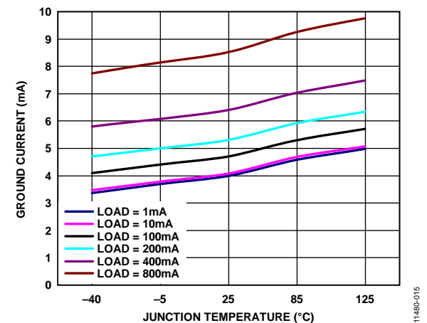
Figure 15. Ground Current vs. Junction Temperature ( T_J ), ADM7151-04, V_{OUT} = 5\text{ V}
