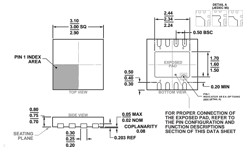
Figure 71. 8-Lead Lead Frame Chip Scale Package [LFCSP] 3 mm x 3 mm Body and 0.75 mm Package Height (CP-8-11)
