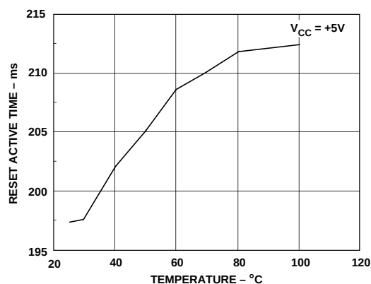
Figure 2. RESET Active Time vs. Temperature
