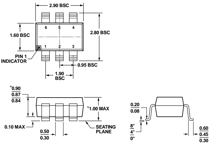
*COMPLIANT TO JEDEC STANDARDS MO-193-AA WITH THE EXCEPTION OF PACKAGE HEIGHT AND THICKNESS. Figure 34. 6-Lead Thin Small Outline Transistor Package [TSOT] (UJ-6) Dimensions shown in millimeters
