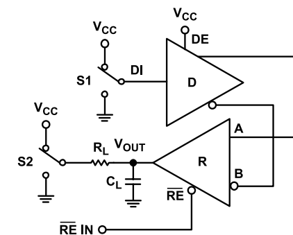
Figure 43. Receiver Enable/Disable from Shutdown
