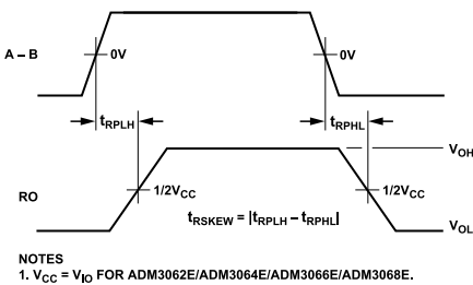
Figure 7. Receiver Propagation Delay Timing Diagram
