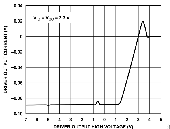
Figure 30. Driver Output Current vs. Driver Output High Voltage
