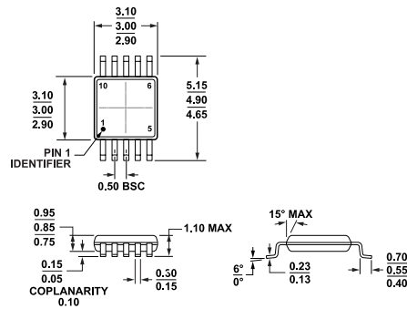
Figure 52. 10-Lead Mini Small Outline Package [MSOP] (RM-10) Dimensions shown in millimeters
