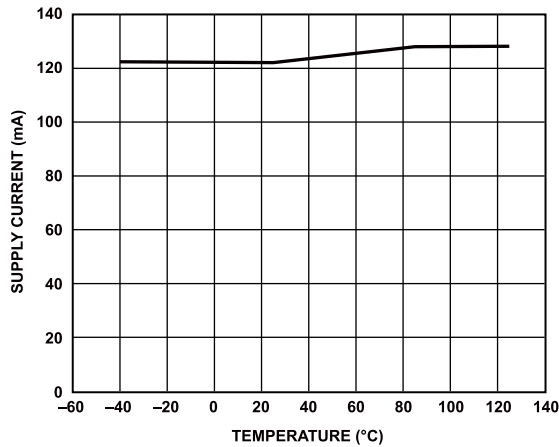
Figure 22. Supply Current ( I_{CC} ) vs. Temperature, Data Rate = 500 kbps, 500 kbps Models, V_{CC} = 5.5 V
