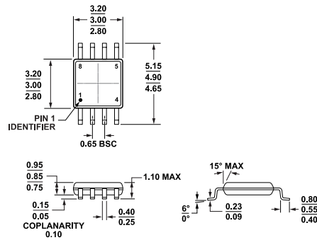
Figure 51. 8-Lead Mini Small Outline Package [MSOP] (RM-8) Dimensions shown in millimeters
