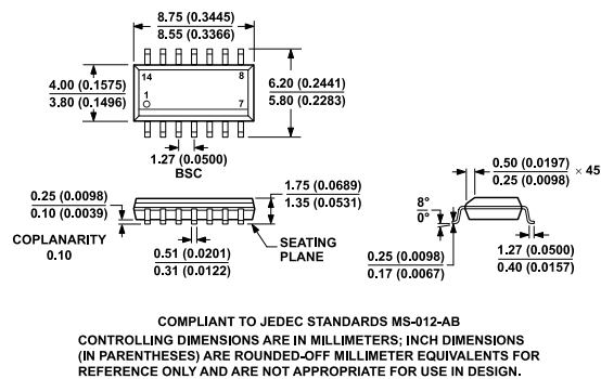
Figure 54. 14-Lead Standard Small Outline Package [SOIC_N] Narrow Body (R-14)
