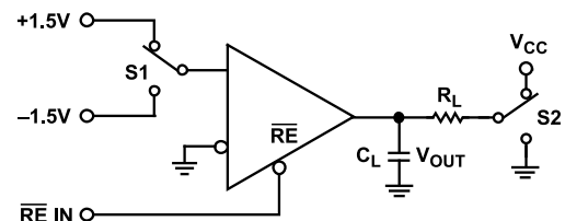
Figure 42. Receiver Propagation Delay/Skew
