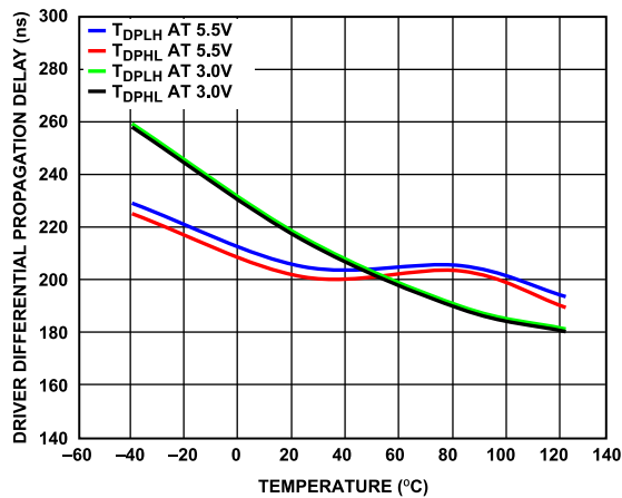
Figure 23. Driver Differential Propagation Delay vs. Temperature, 500 kbps Models
