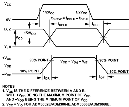
Figure 5. Driver Propagation Delay Rise and Fall Timing Diagram
