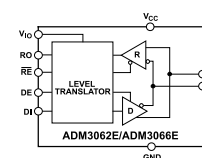
Figure 3. ADM3062E/ADM3066E Functional Block Diagram
