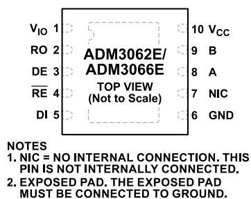
Figure 11. ADM3062E/ADM3066E 10-Lead LFCSP Pin Configuration
