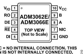
Figure 12. ADM3062E/ADM3066E 10-Lead MSOP Pin Configuration
