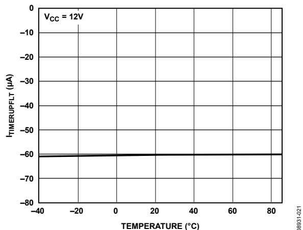
Figure 20. Timer Pull-Up Current, Overcurrent Fault ( I_{\text{TIMERUPFLT}} ) vs. Temperature
