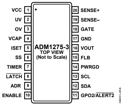
Figure 6. ADM1275-3 Pin Configuration, QSOIP
