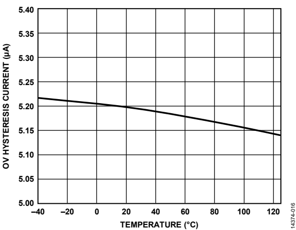
Figure 15. OV Hysteresis Current vs. Temperature
