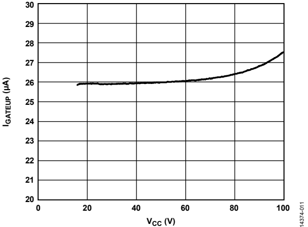
Figure 11. GATE Pull-Up Current ( I_{GATEUP} ) vs. V_{CC}
