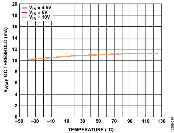
Figure 10. V_{CAP} Overcurrent (OC) Threshold vs. Temperature, Different Input Voltages
