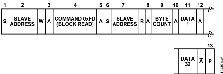
Figure 48. Block Read from the EEPROM or RAM
