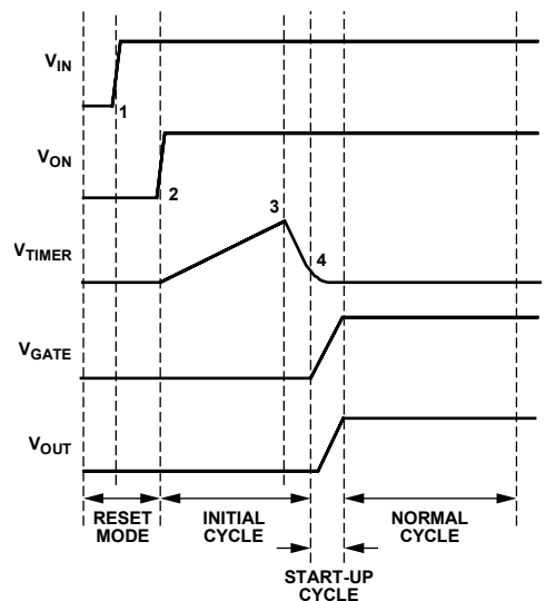
Figure 38. Power-Up Timing
