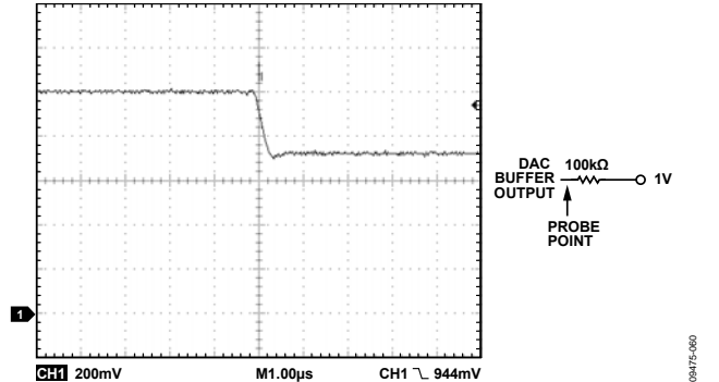
Figure 18. Transient Response of DAC to Turn-On from High-Z State
