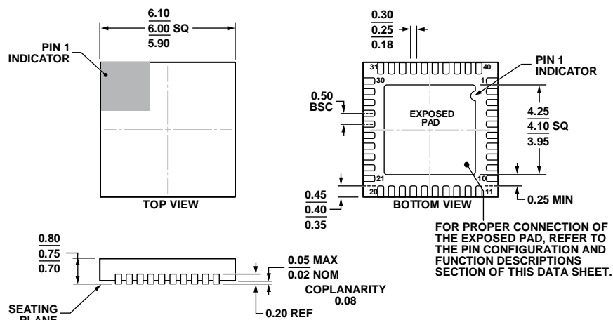
Figure 48. 40-Lead Frame Chip Scale Package [LFCSP_WQ] 6 mm × 6 mm Body, Very Very Thin Quad (CP-40-9) Dimensions shown in millimeters
