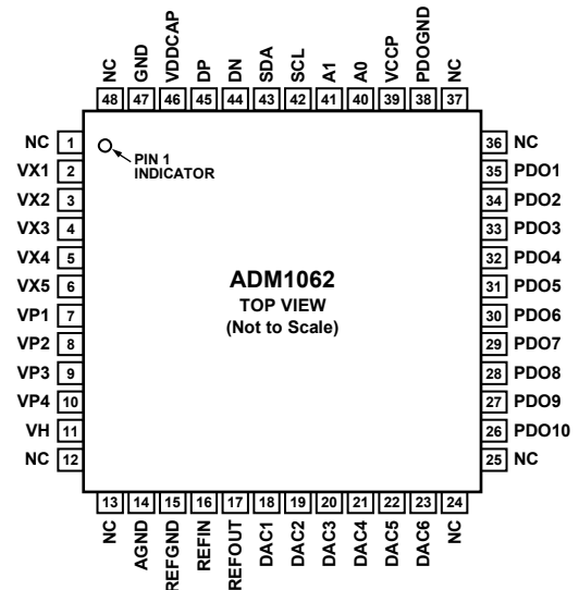
Figure 4. 48-Lead TQFP Pin Configuration
