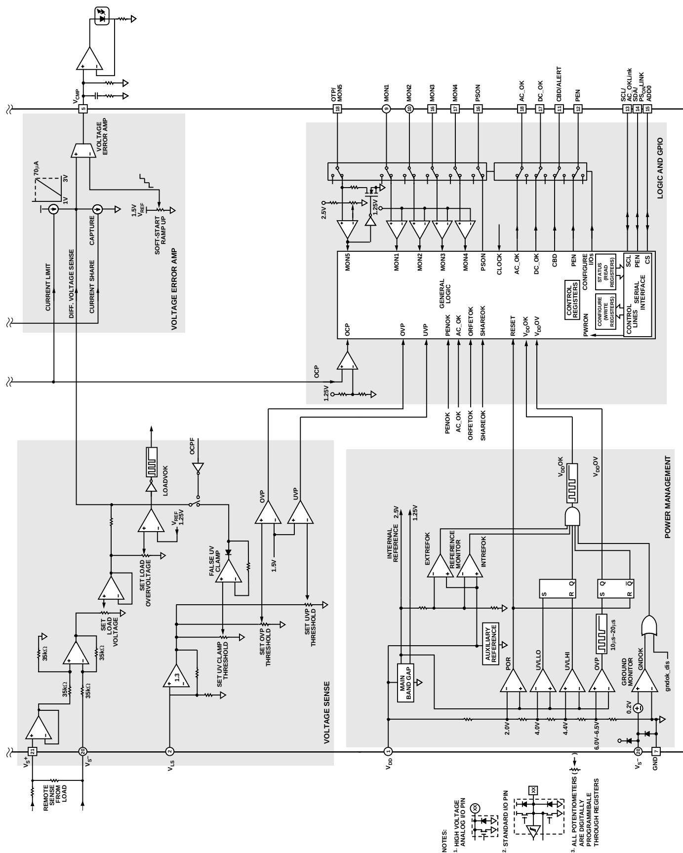
Figure 4. ADM1041A Diagram, Part 2
