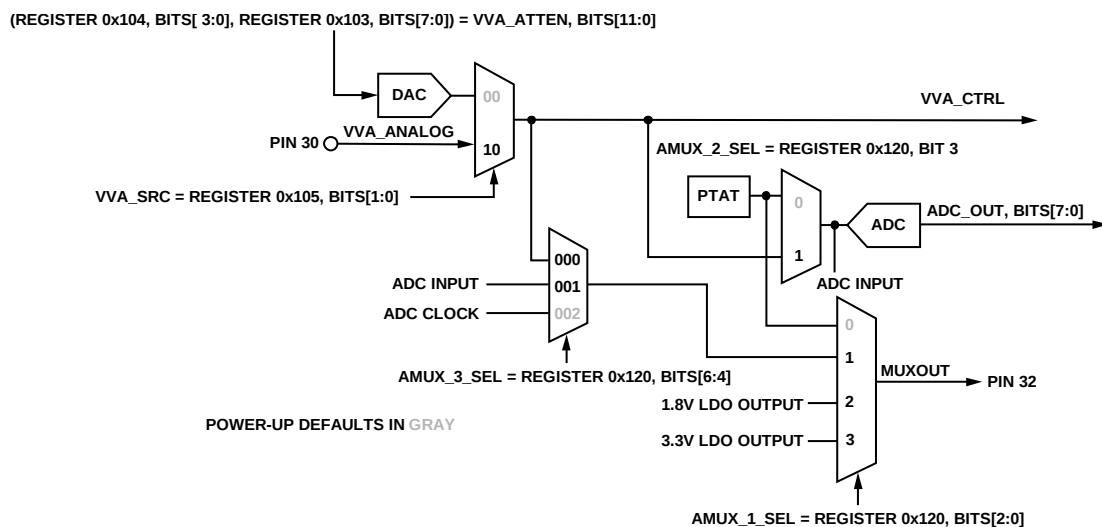
Figure 41. Auxiliary Mux Block Diagram
