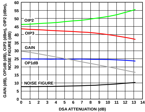
Figure 22. Gain, OP1dB, OIP3, OIP2, Noise Figure vs. DSA Attenuation; VVA Attenuation = 0 dB, Frequency = 620 MHz
