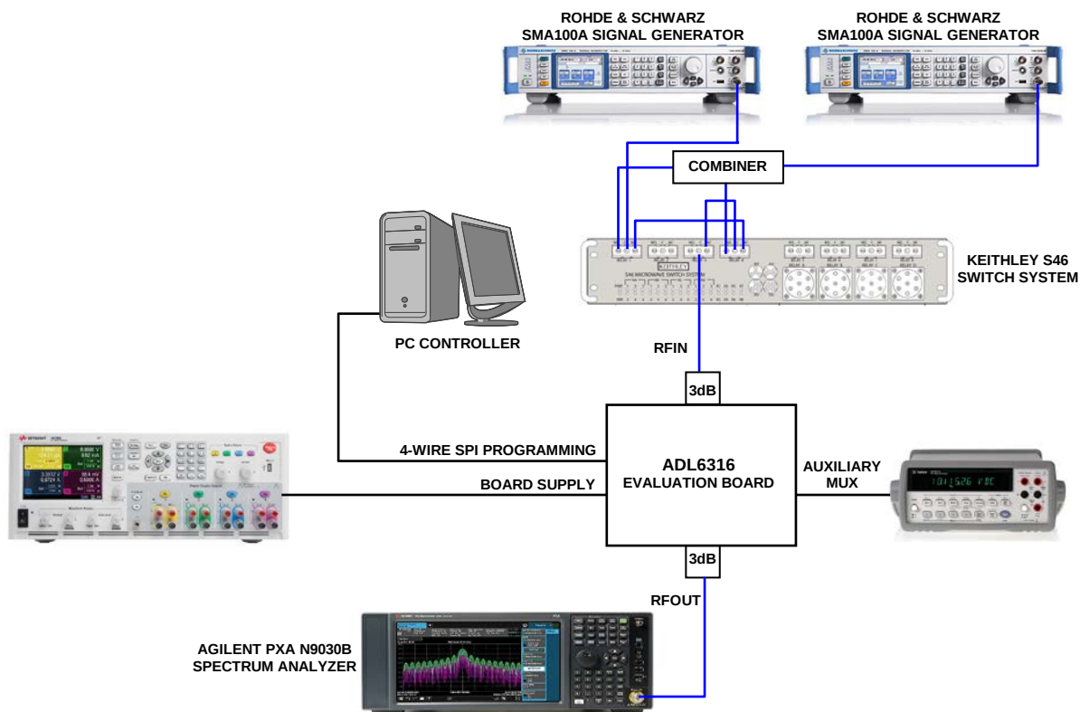
Figure 49. General Characterization Setup
