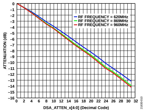
Figure 10. Attenuation vs. DSA_ATTEN_x[4:0] at 620 MHz, 869 MHz, and 960 MHz; VVA Attenuation = 0\text{ dB}
