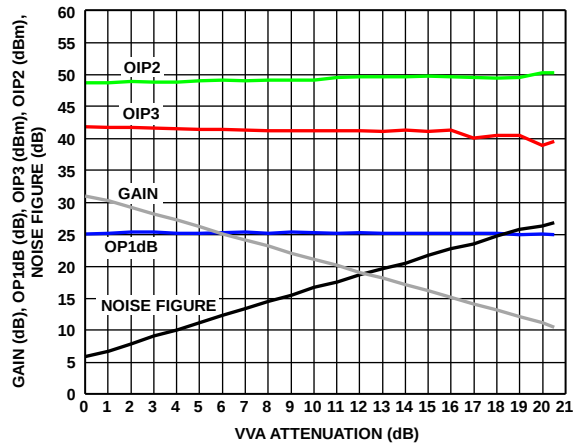
Figure 23. Gain, OP1dB, OIP3, OIP2, Noise Figure vs. VVA Attenuation; DSA Attenuation = 0 dB, Frequency = 869 MHz
