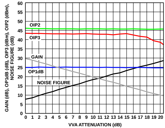
Figure 21. Gain, OP1dB, OIP3, OIP2, Noise Figure vs. VVA Attenuation; DSA Attenuation = 0 dB, Frequency = 620 MHz
