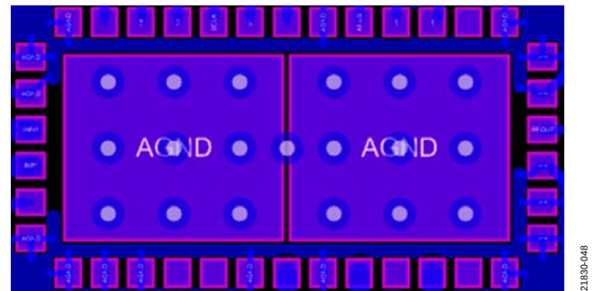
Figure 48. Evaluation Board Layout for the ADL6316-EVALZ
