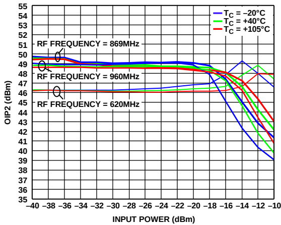
Figure 18. OIP2 vs. Input Power for Various Temperatures at 620 MHz, 869 MHz, and 960 MHz
