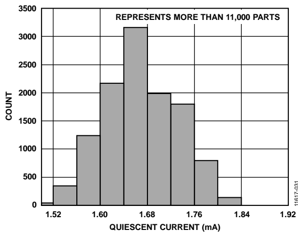
Figure 32. Distribution of Quiescent Current at 25°C
