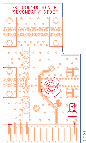
Figure 49. ADL6010 Evaluation Board Layout, Bottom Side
