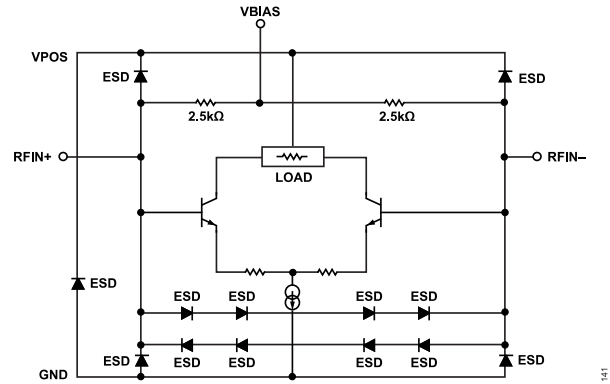
Figure 42. RF Inputs
