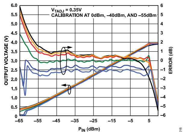
Figure 16. V_{RMS} and Log Conformance Error vs. Input Level and Temperature at 2.14 GHz
