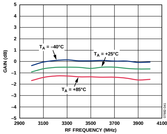
Figure 41. Power Conversion Gain vs. RF Frequency
