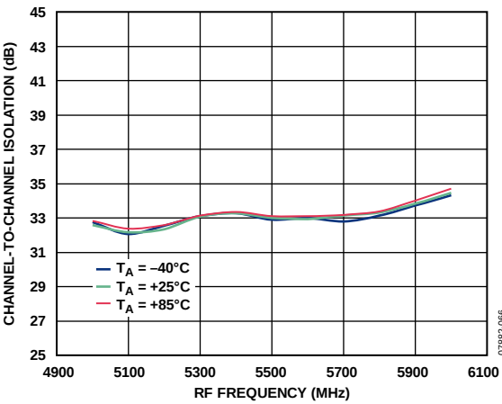
Figure 66. Channel-to-Channel Isolation
