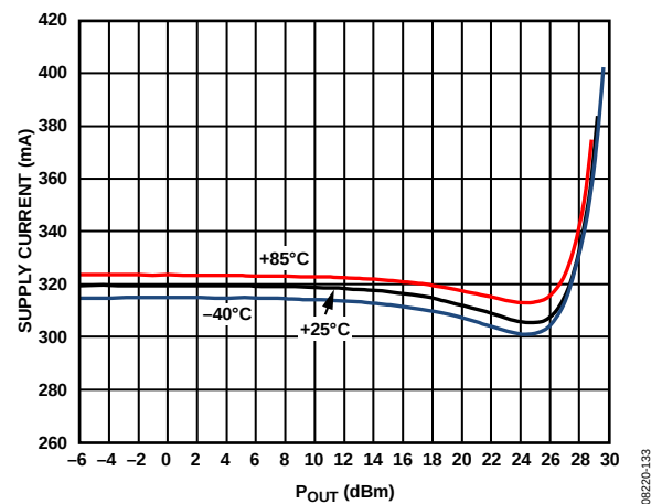
Figure 33. Supply Current vs. P_{OUT} and Temperature, V_{CC} = 5\text{ V} at 2140 MHz
