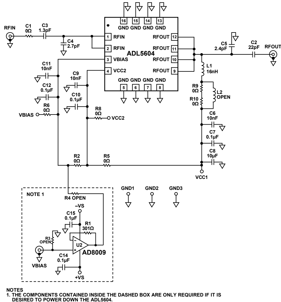
Figure 36. Basic Connections
