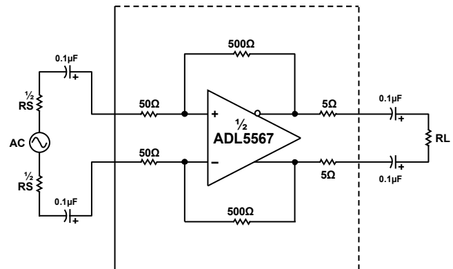
Figure 38. Basic Structure
