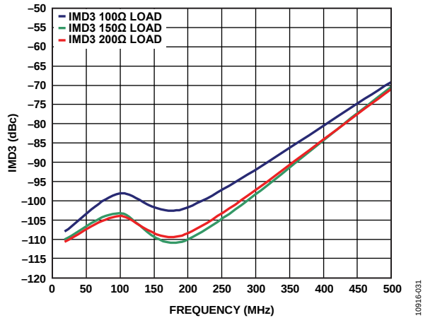
Figure 15. IMD3 vs. Frequency, R_L = 100\Omega , R_L = 150\Omega , and R_L = 200\Omega , V_{POS} = 3.3\text{ V} , Input Common-Mode = 1.65 V, Output Common-Mode = 1.25 V, V_{OUT} = 1.5\text{ V p-p}
