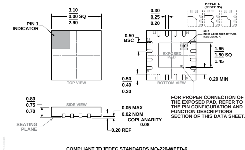
Figure 48. 16-Lead Lead Frame Chip Scale Package [LFCSP] 3 mm × 3 mm Body and 0.75 mm Package Height (CP-16-27) Dimensions shown in millimeters
