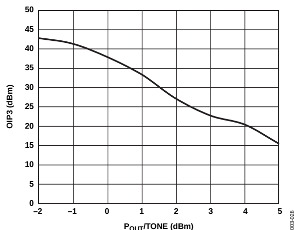
Figure 13. Output Third-Order Intercept (OIP3) vs. Power ( P_{OUT} ), Frequency 140 MHz, A_V = 15.5 dB
