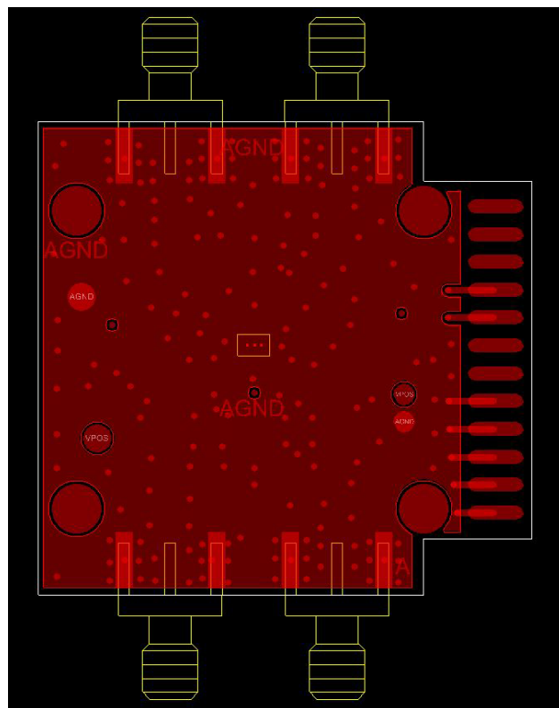
Figure 27. Evaluation Board Layout, Bottom Layer
