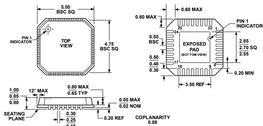
Figure 77. 32-Lead Lead Frame Chip Scale Package [LFCSP_VQ] 5 mm × 5 mm Body, Very Thin Quad Lead (CP-32-8) Dimensions shown in millimeters
