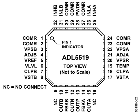
Figure 2. Pin Configuration
