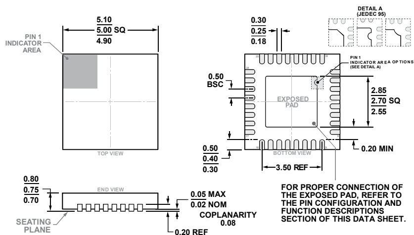
Figure 77. 32-Lead Lead Frame Chip Scale Package [LF CSP] 5 mm x 5 mm Body and 0.75 mm Package Height (CP-32-21)
