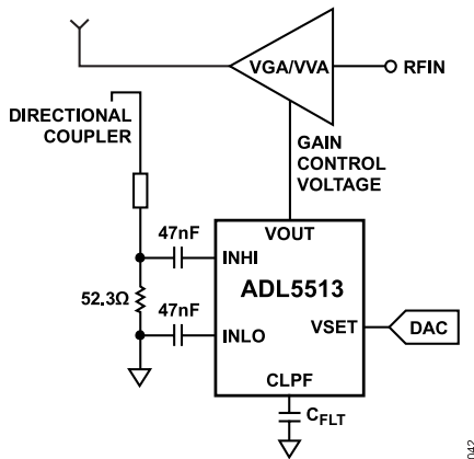
Figure 42. Controller Mode
