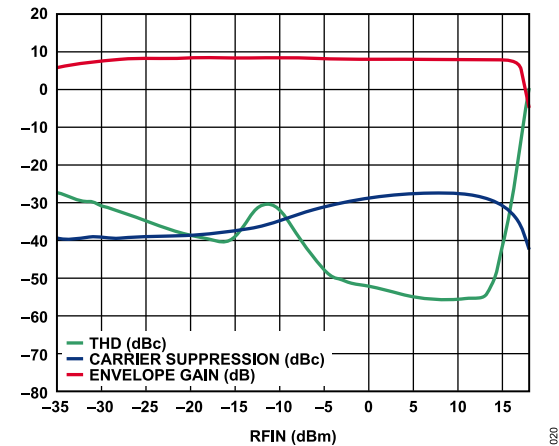
Figure 36. THD on V_{ENV} vs. RF Input Level; 1900 MHz RF Input, AM Modulated by a 20 MHz Sine Wave (Modulation Index = 0.25), V_{ENV} Output AC-Coupled into a 50 Ω Spectrum Analyzer Load
