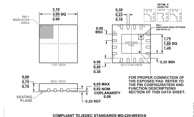
Figure 62. 16-Lead Lead Frame Chip Scale Package [LFCSP] 3 mm x 3 mm Body and 0.75 mm Package Height (CP-16-22) Dimensions shown in millimeters
