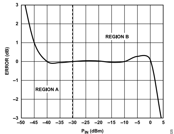
Figure 45. Error vs. P_{IN}
