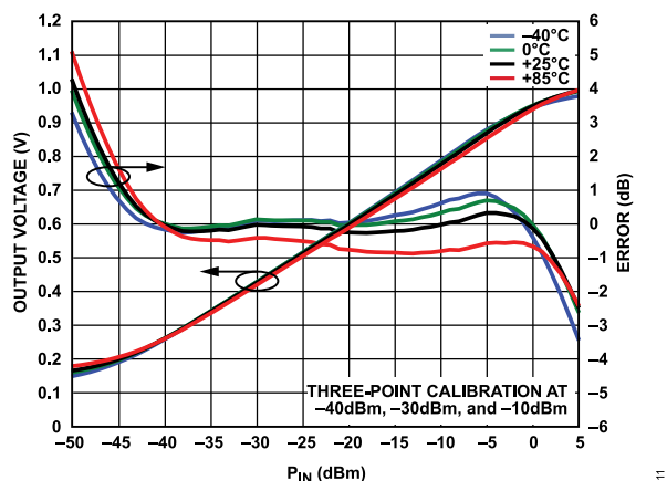
Figure 11. V_{LOG} and Log Conformance Error vs. P_{IN} over Temperature at 100 MHz
