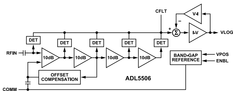
Figure 41. Block Schematic
