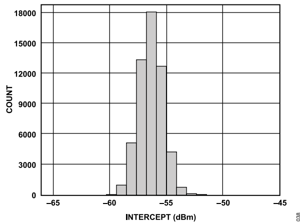
Figure 34. Distribution of Intercept at 900 MHz, 25°C
