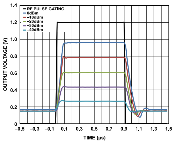
Figure 29. Output Response to RF Burst Input for Various RF Input Levels, Carrier Frequency = 100 MHz, C_{FLT} = Open (See Figure 40 in the Measurement Setups Section)
