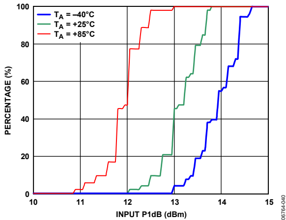
Figure 44. IP1dB Distributions
