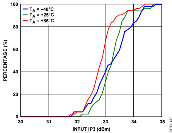
Figure 31. IIP3 Distributions
