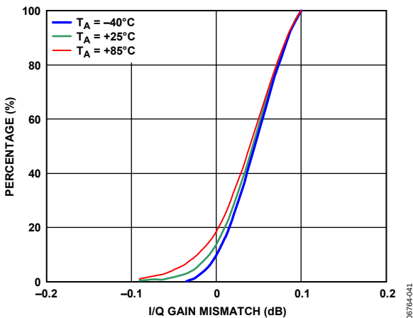
Figure 45. I/Q Gain Mismatch Distributions
