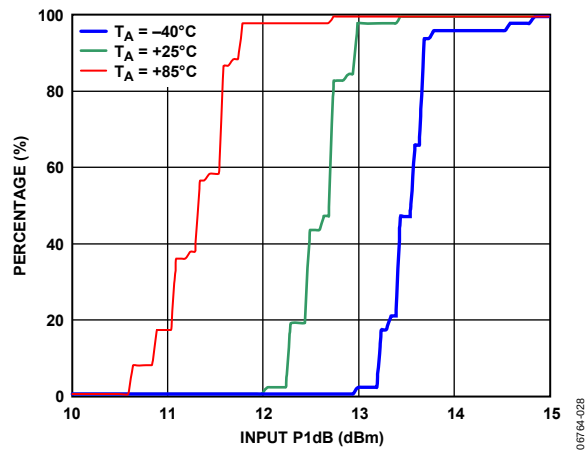
Figure 32. IP1dB Distributions
