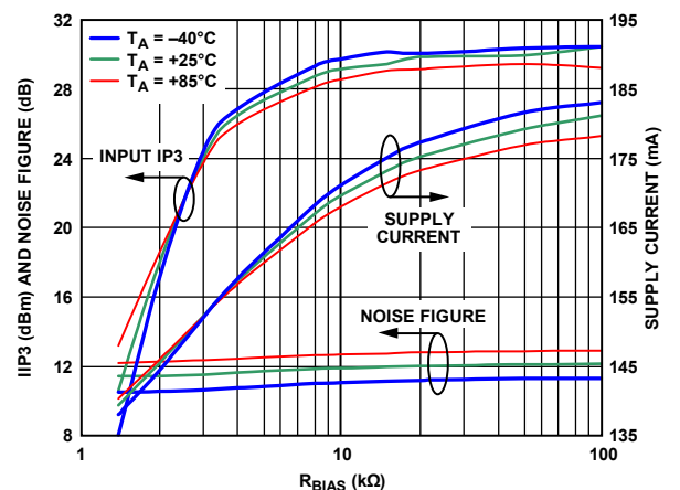
Figure 14. Noise Figure, IIP3, and Supply Current vs. R_{BIAS} , f_{RF} = 140 MHz
