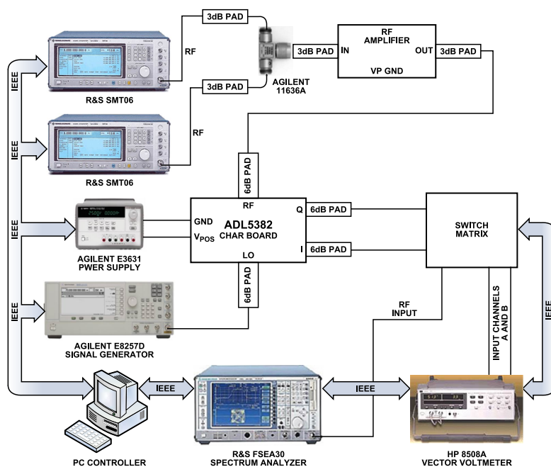
Figure 59. General Characterization Setup
