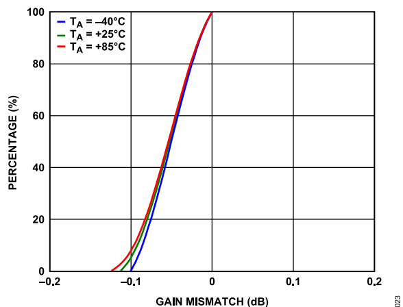
Figure 23. IQ Gain Mismatch Distributions, f_{RF} = 900 \text{ MHz}
