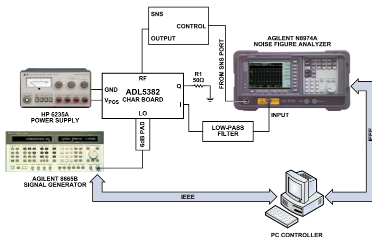
Figure 57. General Noise Figure Measurement Setup
