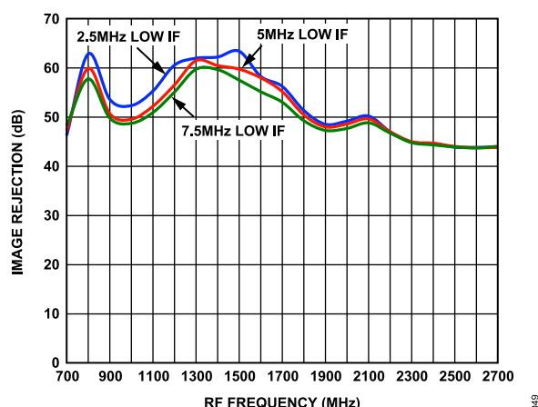
Figure 49. Image Rejection vs. RF Frequency for a W-CDMA Signal, IF = 2.5 MHz, 5 MHz, and 7.5 MHz
