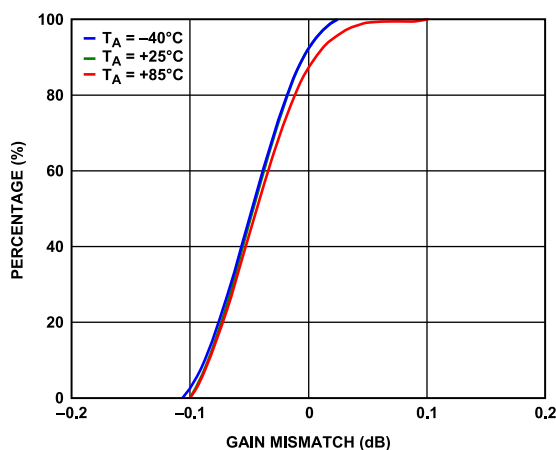
Figure 29. IQ Gain Mismatch Distributions, f_{RF} = 1900 MHz
