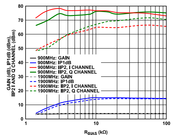
Figure 14. Conversion Gain, IP1dB, IIP2_I, and IIP2_Q vs. R_{BIAS} , f_{RF} = 900 \text{ MHz} , 1900 \text{ MHz}
