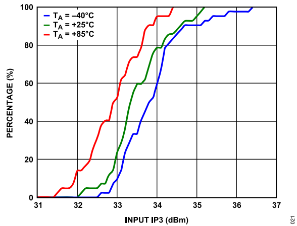
Figure 21. IIP3 Distributions, f_{RF} = 900 \text{ MHz}
