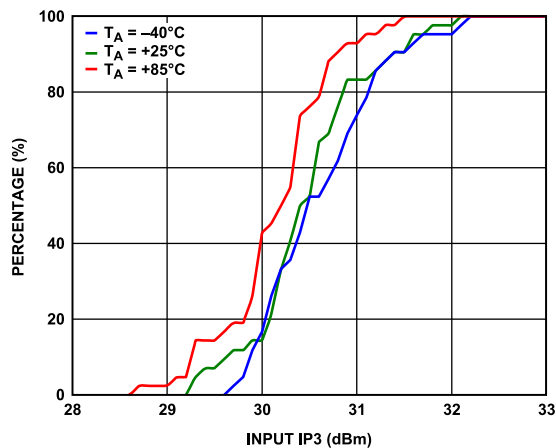
Figure 27. IIP3 Distributions, f_{RF} = 1900 MHz
