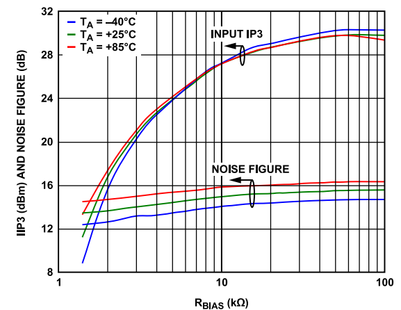
Figure 13. IIP3 and Noise Figure vs. R_{BIAS} , f_{RF} = 1900 \text{ MHz}
