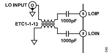
Figure 40. Differential LO Drive
