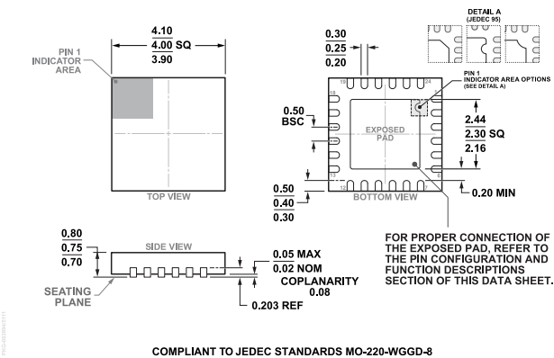
Figure 65. 24-Lead Lead Frame Chip Scale Package [LFCSP] 4 mm x 4 mm Body and 0.75 mm Package Height (CP-24-14) Dimensions shown in millimeters
