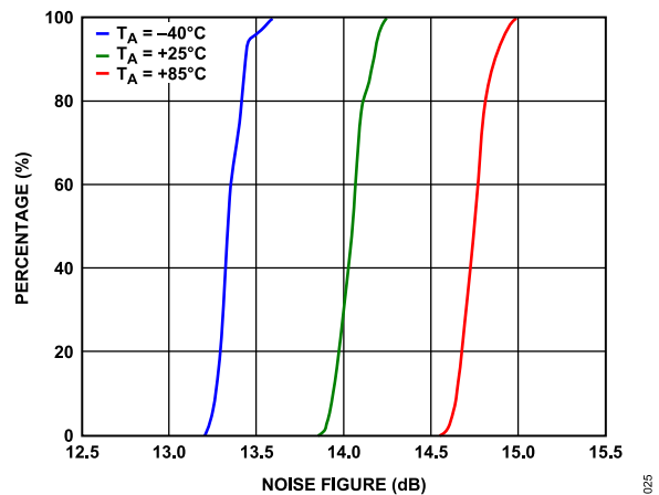
Figure 25. Noise Figure Distributions, f_{RF} = 900 \text{ MHz}
