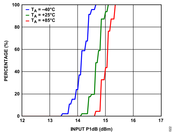
Figure 22. IP1dB Distributions, f_{RF} = 900 \text{ MHz}
