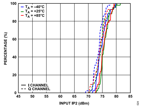
Figure 24. IIP2 Distributions for I Channel and Q Channel, f_{RF} = 900 \text{ MHz}
