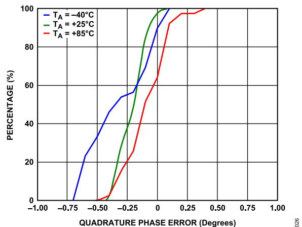
Figure 26. IQ Quadrature Phase Error Distributions, f_{RF} = 900 \text{ MHz}
