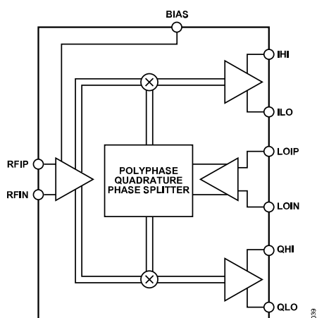
Figure 39. Block Diagram
