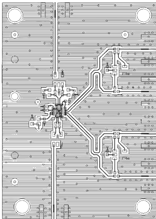
Figure 61. Evaluation Board Top Layer
