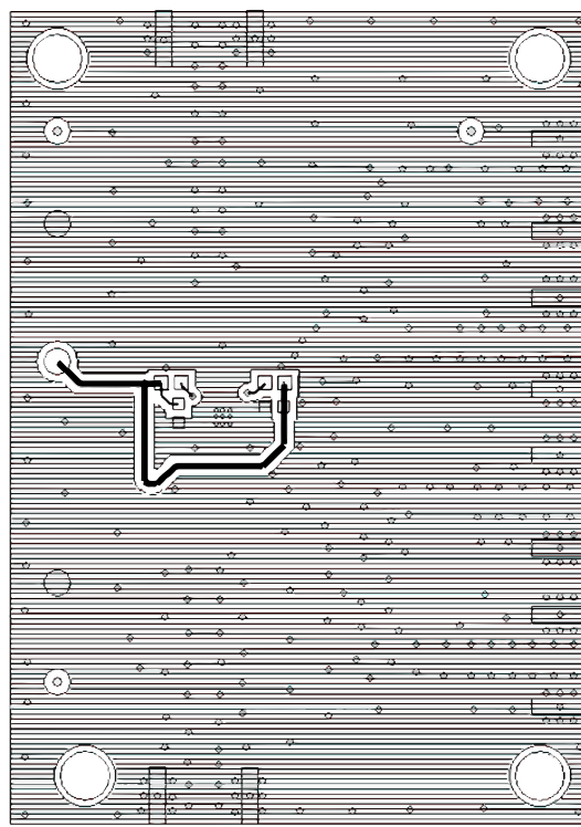
Figure 63. Evaluation Board Bottom Layer
