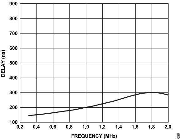
Figure 56. Fourth-Order Low-Pass W-CDMA Filter Group Delay Response
