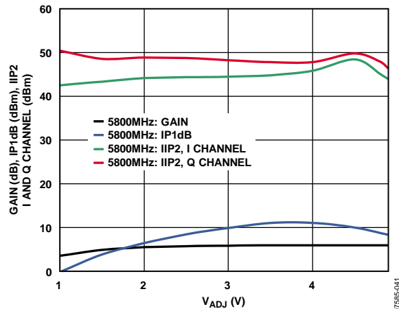
Figure 41. Conversion Gain, IP1dB, and IIP2 vs. V_{ADJ} , f_{LO} = 5800\text{ MHz}
