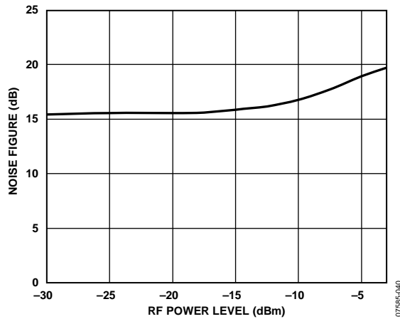
Figure 40. Noise Figure vs. Input Blocker Level, f_{LO} = 5800\text{ MHz} (RF Blocker 5 MHz Offset)
