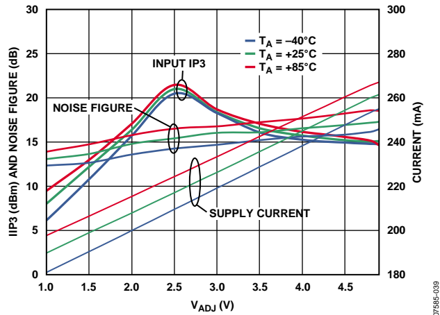
Figure 39. IIP3, Noise Figure, and Supply Current vs. V_{ADJ} , f_{LO} = 5800\text{ MHz}
