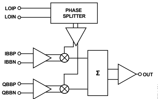
Figure 24. Block Diagram
