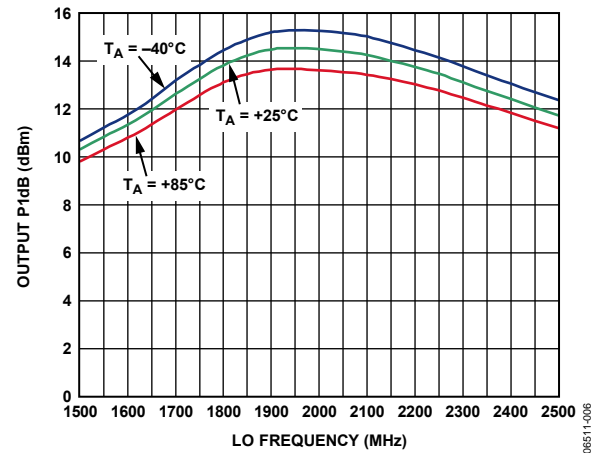
Figure 6. SSB Output P1dB Compression Point (OP1dB) vs. f_{\text{LO}} and Temperature
