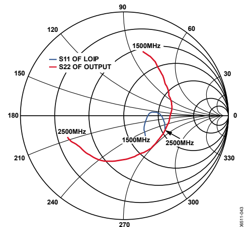
Figure 8. Smith Chart of LOIP S11 and VOUT S22 ( f_{\text{LO}} from 1600 MHz to 2500 MHz)
