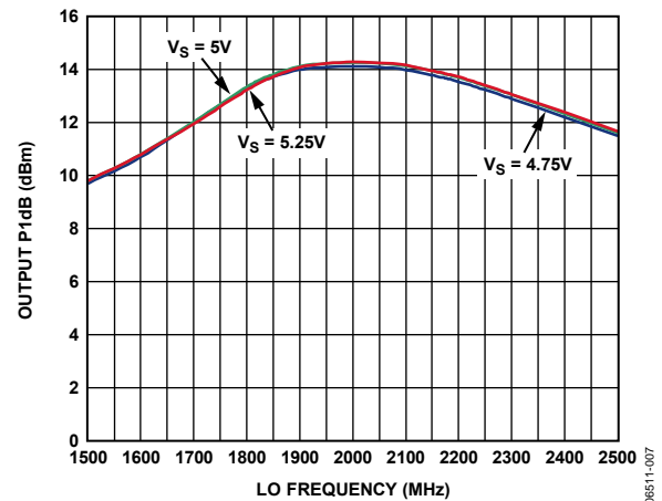
Figure 7. SSB Output P1dB Compression Point (OP1dB) vs. f_{\text{LO}} and Supply
