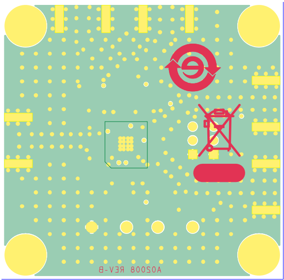
Figure 50. Evaluation Board Bottom Layer
