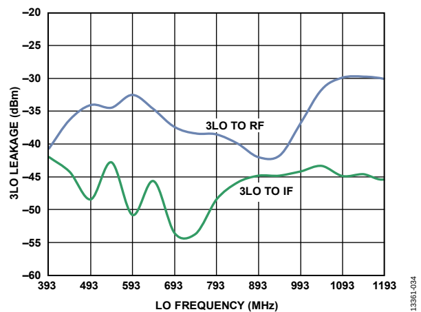
Figure 33. 3LO Leakage vs. LO Frequency
