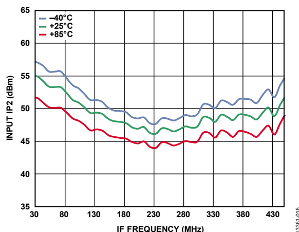
Figure 16. Input IP2 vs. IF Frequency
