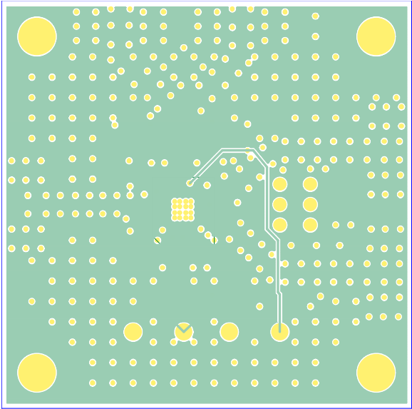
Figure 49. Evaluation Board Power Plane, Internal Layer 2
