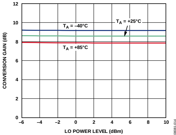
Figure 21. Power Conversion Gain vs. LO Power
