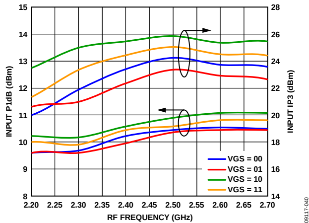
Figure 40. Input IP3 and Input P1dB vs. RF Frequency
