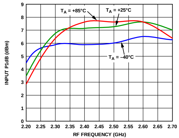
Figure 47. Input P1dB vs. RF Frequency at 3.3 V
