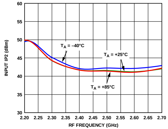
Figure 46. Input IP2 vs. RF Frequency at 3.3 V
