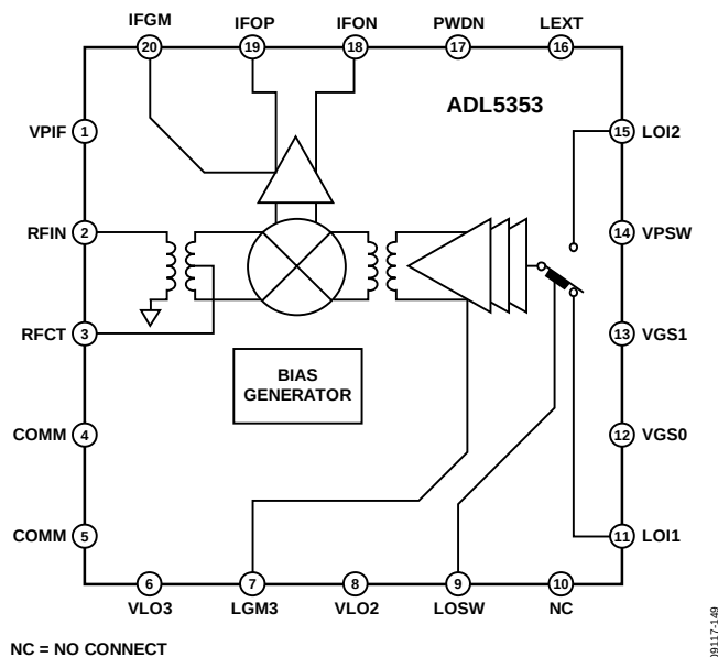
Figure 49. Simplified Schematic
