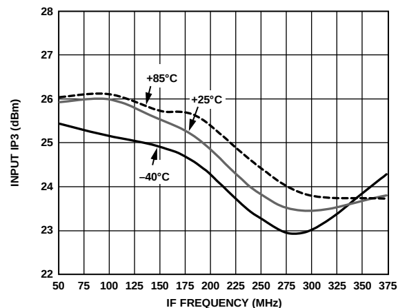
Figure 46. Input IP3 vs. IF Frequency
