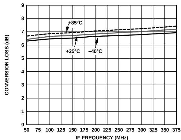
Figure 45. Conversion Loss vs. IF Frequency
