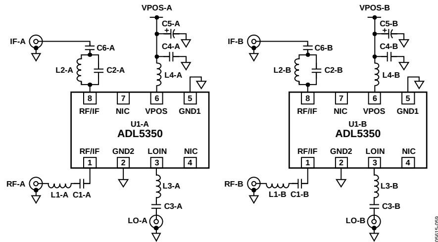
Figure 65. Evaluation Board
