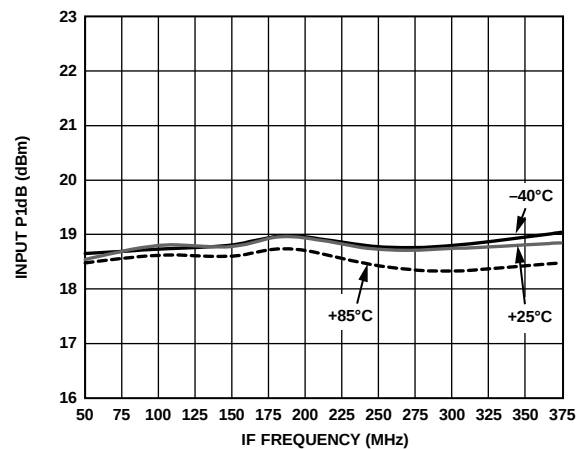
Figure 47. Input P1dB vs. IF Frequency
