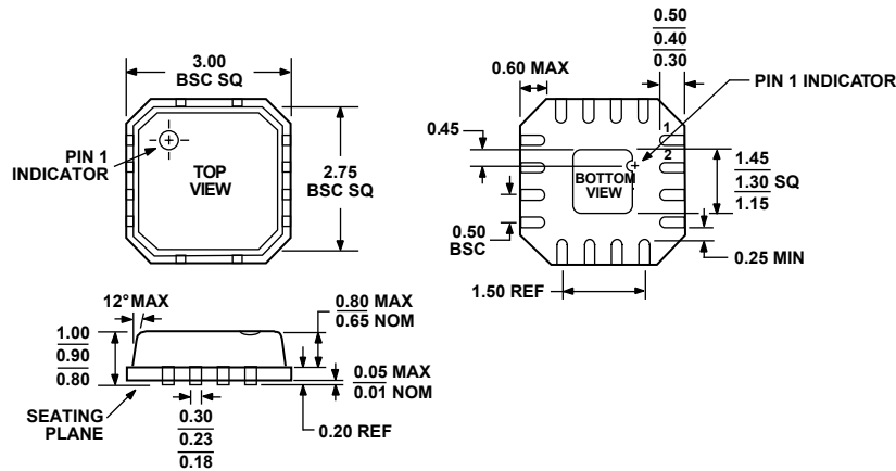
COMPLIANT TO JEDEC STANDARDS MO-220-VEED-2 Figure 32. 16-Lead Leadframe Chip Scale Package [LFCSP] (CP-16) Dimensions shown in millimeters
