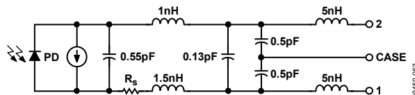
Figure 54. Photodiode Model
