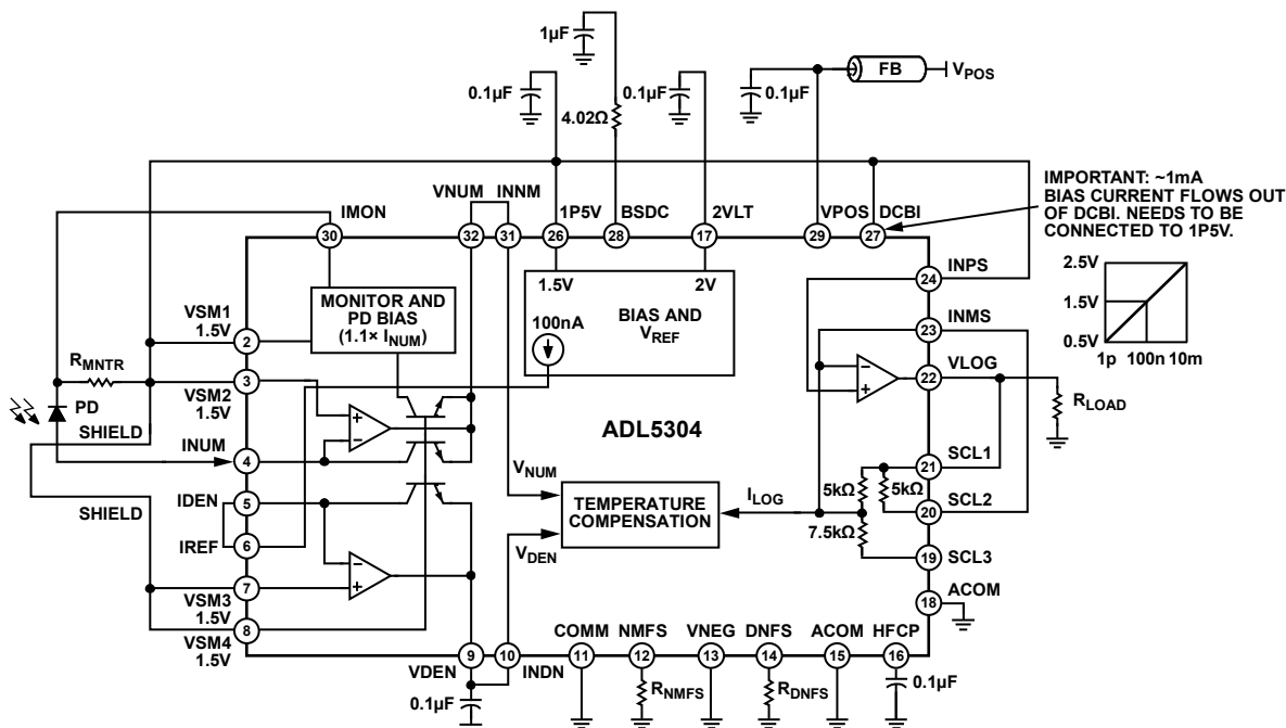
Figure 55. Basic Connections for Single-Supply Operation
