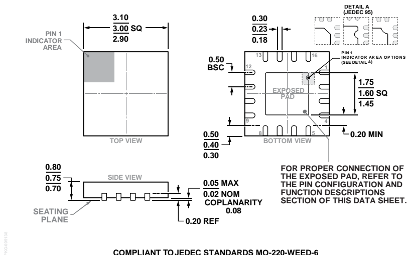
Figure 34. 16-Lead Lead Frame Chip Scale Package [LFCSP] 3 mm × 3 mm Body and 0.75 mm Package Height (CP-16-22) Dimensions shown in millimeters
