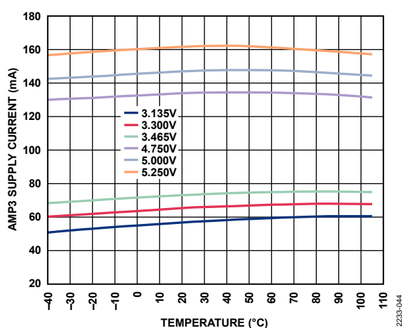
Figure 62. AMP3 Supply Current vs. Temperature by Voltage
