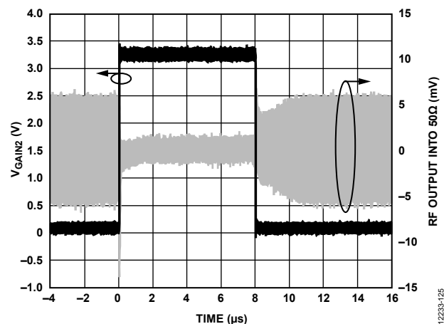
Figure 25. AMP2 Typical Output Response with 3.3 V Step on V_{GAIN2} , V_{GAIN1} = 3.3 V, HG Mode, 0.9 GHz
