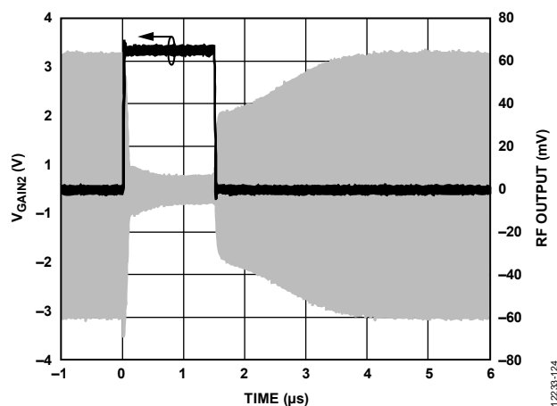
Figure 24. AMP2 Typical Output Response with 3.3 V Step on V_{GAIN2} , V_{GAIN1} = 0 V, HG Mode, 0.9 GHz
