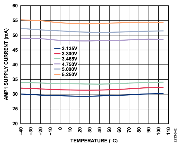
Figure 60. AMP1 Supply Current vs. Temperature by Voltage
