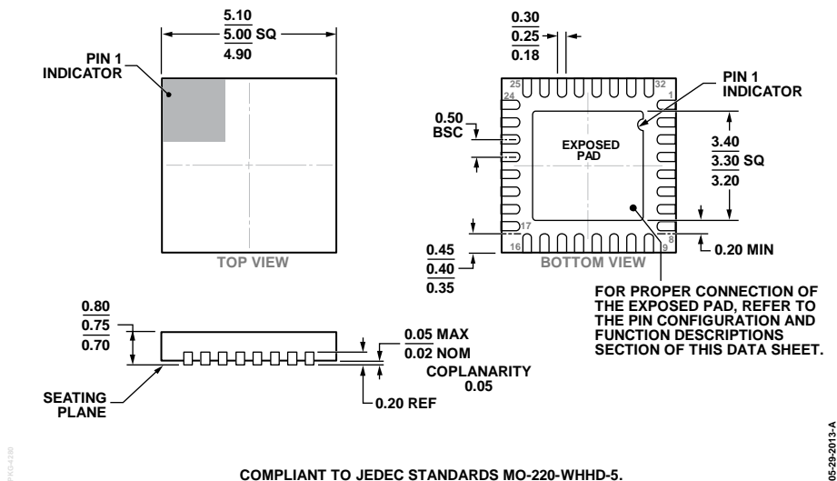
COMPLIANT TO JEDEC STANDARDS MO-220-WHHD-5. Figure 85. 32-Lead Lead Frame Chip Scale Package [LFCSP_WQ] 5 mm × 5 mm Body, Very Very Thin Quad (CP-32-20) Dimensions shown in millimeters
