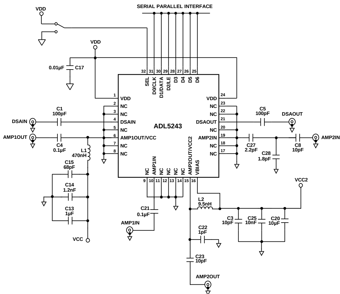
Figure 58. Basic Connections
