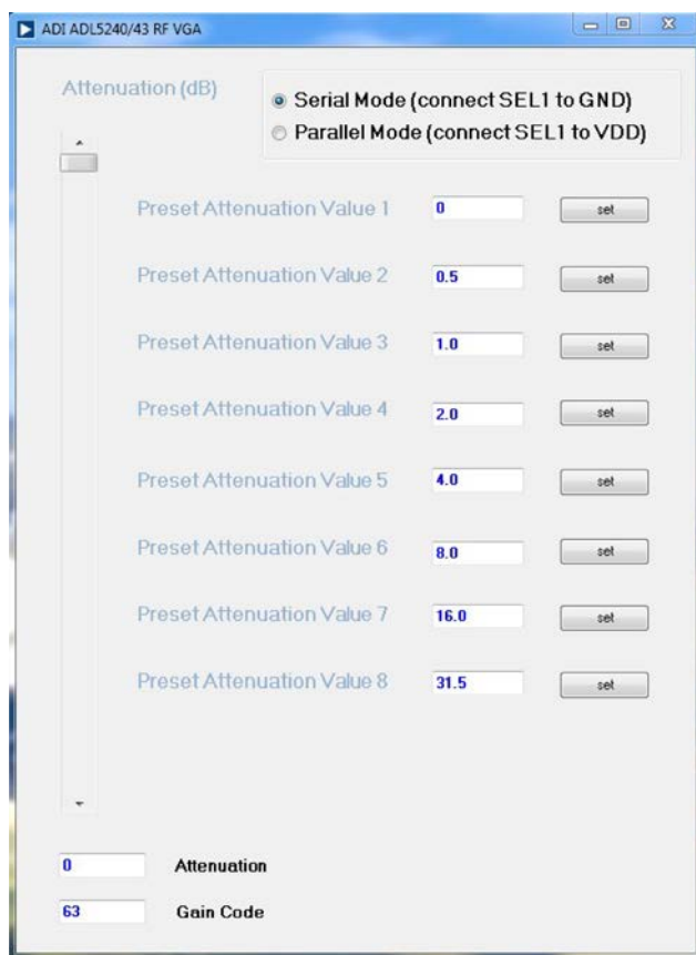
Figure 45. Evaluation Board Control Software
