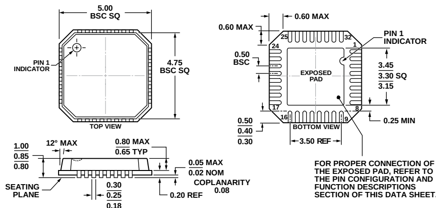
COMPLIANT TO JEDEC STANDARDS MO-220-VHHD-2 Figure 46. 32-Lead Lead Frame Chip Scale Package [LFCSP_VQ] 5 mm x 5 mm Body, Very Thin Quad (CP-32-3) Dimensions shown in millimeters
