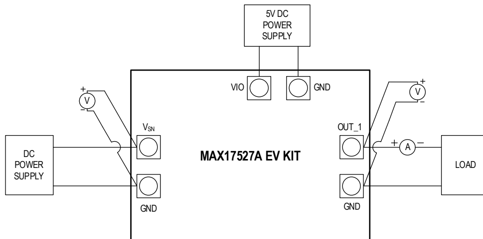
Figure 1. MAX17527A EV Kit Setup Diagram
