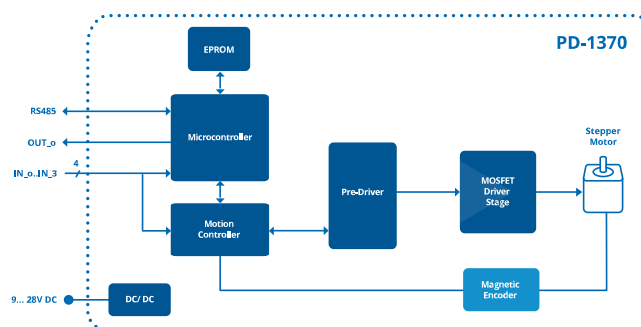
Figure 13: PD42-x-1370 block diagram
