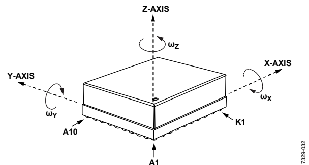
Figure 49. Gyroscope Axis and Polarity Assignments
