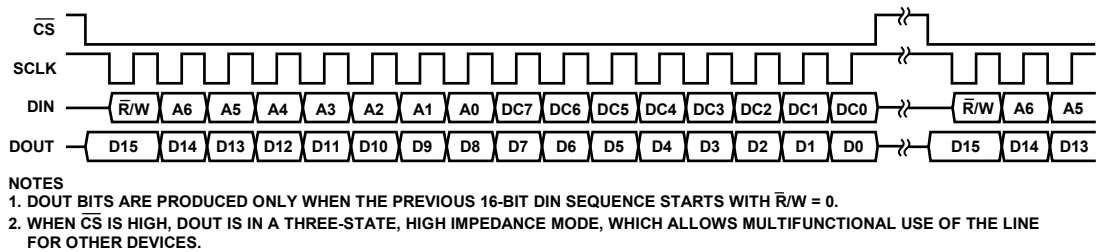
Figure 41. SPI Communication Bit Sequence
