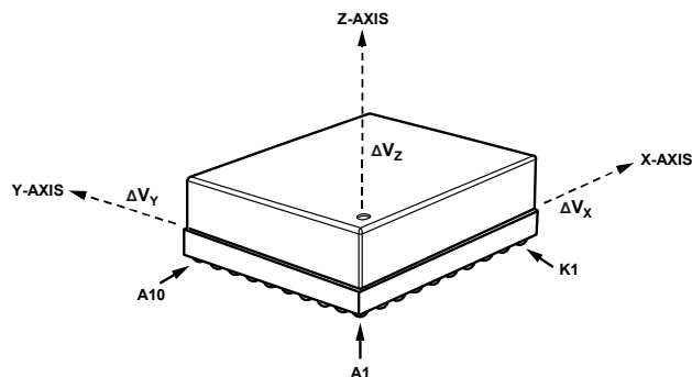
Figure 55. Delta Velocity Axis and Polarity Assignments
